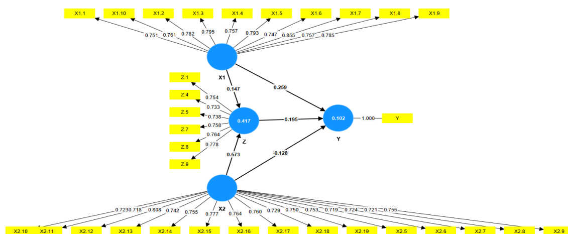
Figure 3.1 PLS-SEM Results
